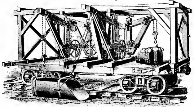
Fig. 217. RAILROAD DITCHING CAR, THE AMERICAN.
